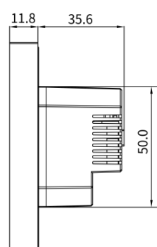
② RIGHT VIEW
